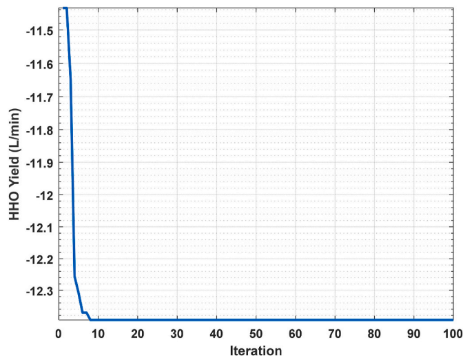
Fig. 11. Convergence of PSO for HHO yield.
